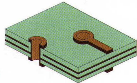
Illustration ML-13. Strip etch resist. The tin or tin/lead is chemically removed.
