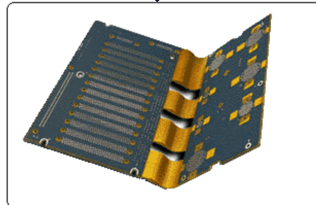
Flexible PCB
